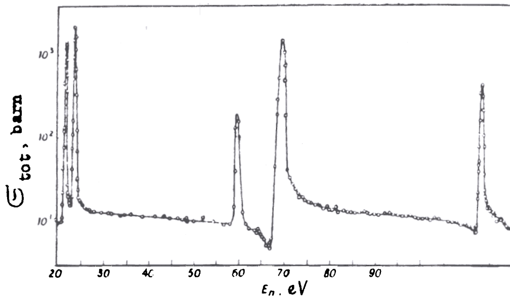
Fig. 1. Resonances in the energy dependence of the total neutron cross section of ^{232}\text{Th} [10].
