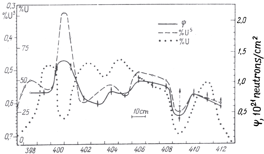
Fig. 4. Distribution of the integrated neutron flux \psi , ^{235}\text{U} concentration in uranium and the concentration of uranium in the ore. Sample numbers are plotted along the abscissa axis. [18]
