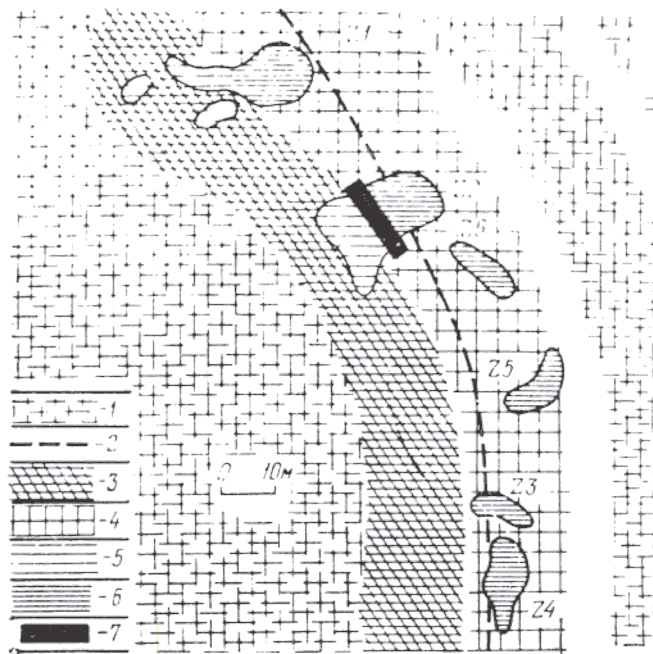
Fig. 3. Disposition of the active zones in the Oklo reactor [18]: 1 - sandstone; 2 - boundary of mined ore; 3 - sandstone wall; 4 - floor of pit; 5 - mined part of reactor; 6 - explored part of reactor; 7 - area to be preserved for future studies.
